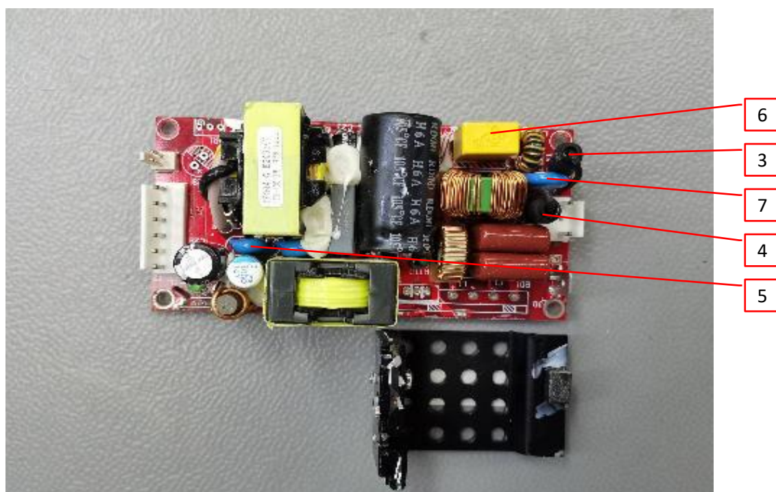
Photo 10 - PCB view
