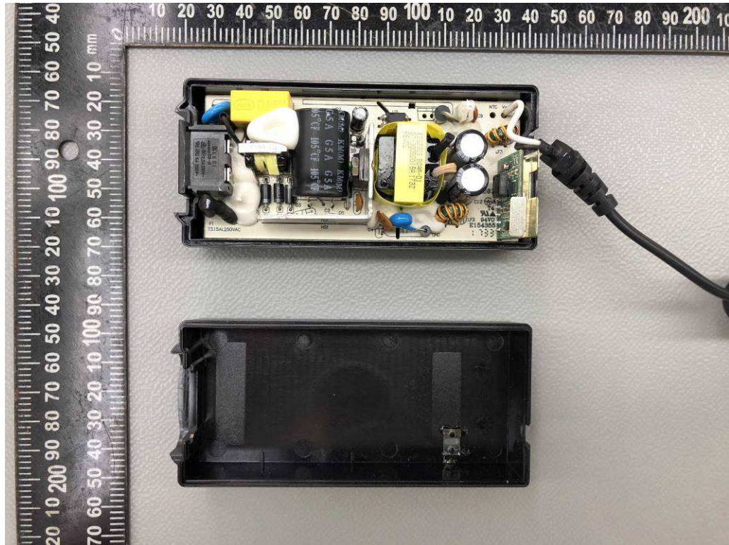
Internal view for GTM91128LI1CEL-****
