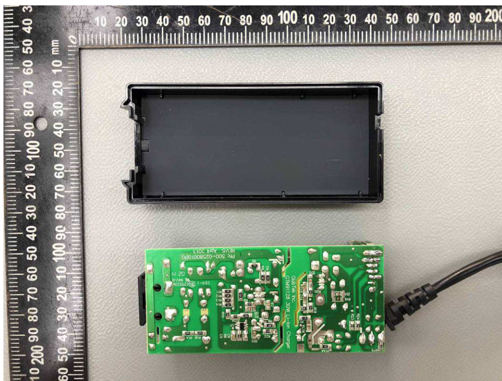
Internal view for GTM91128LI1CELM-****
