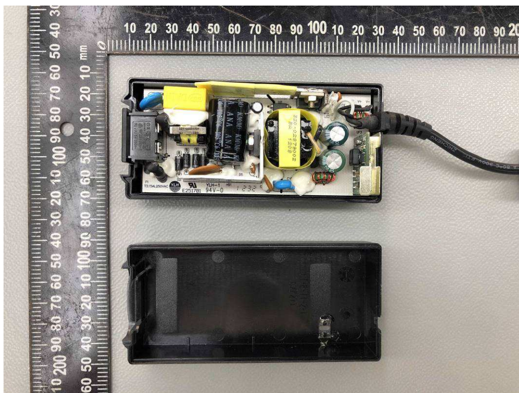
Internal view for GTM91128LI3CELM-**** or GTM91128*DUALC-****
