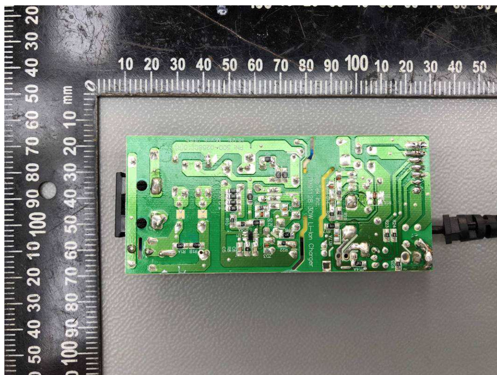
PCB for GTM91128LI1CEL-****
