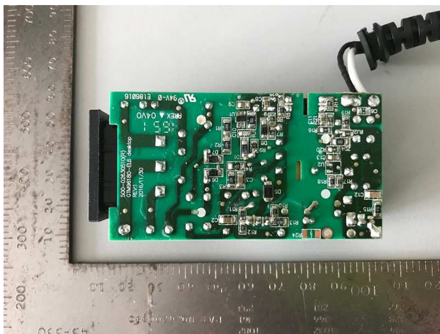
PCB view for GTM96180 series (Class I) without R22, R23 and R24
