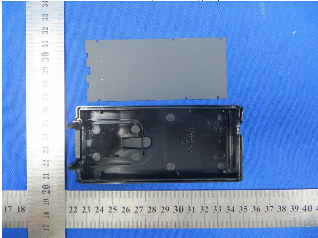
Internal view (Enclosure Type 2)
