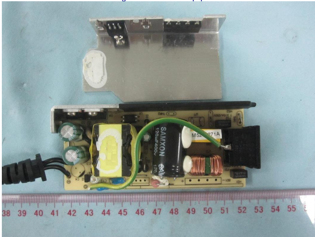
Earthing wire for Class I equipment
