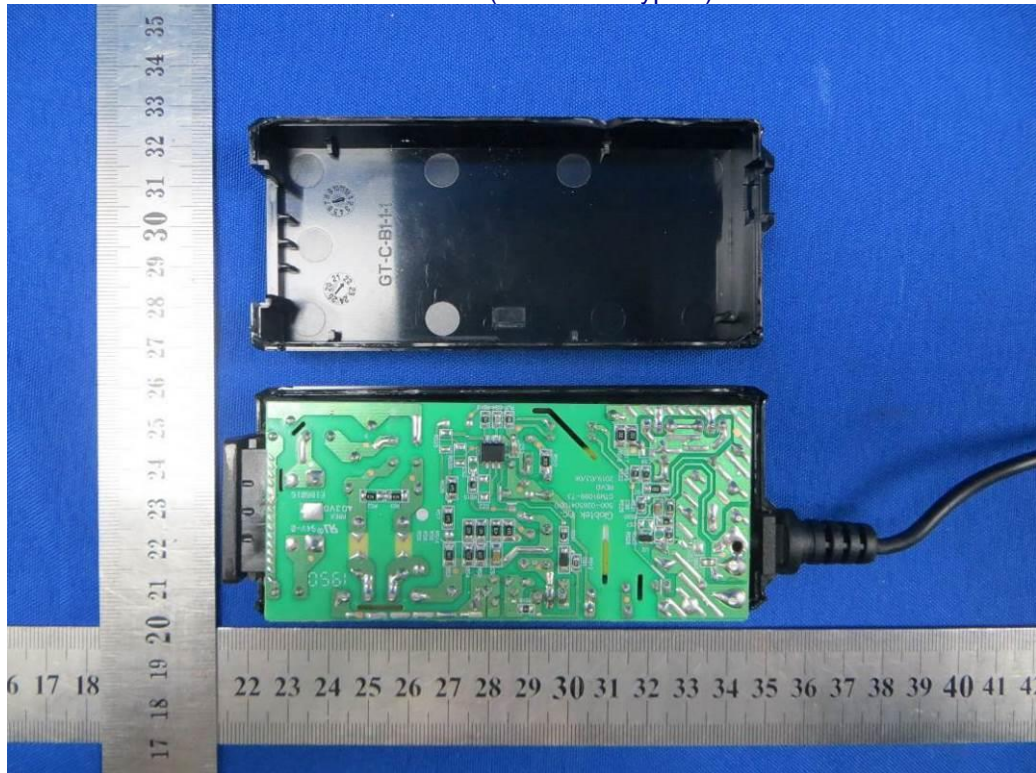
Internal view (Enclosure Type 1)
