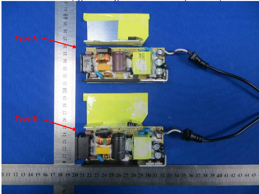
PCB view (Type A and Type B are same on component side)
