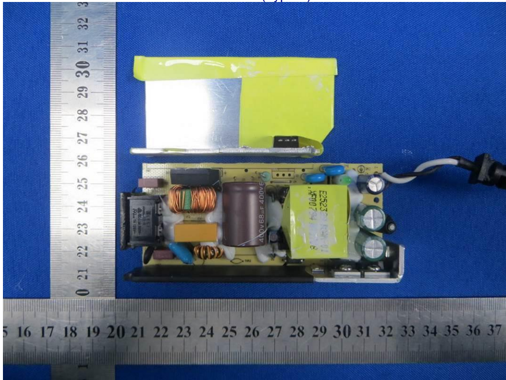
PCB view (Type A)
