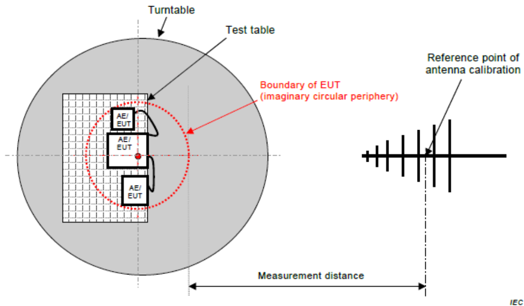
Figure C.1 – Measurement distance
