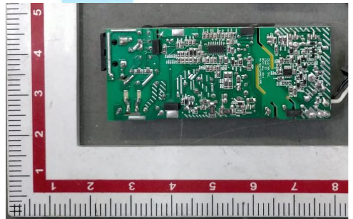
PCB Back View
